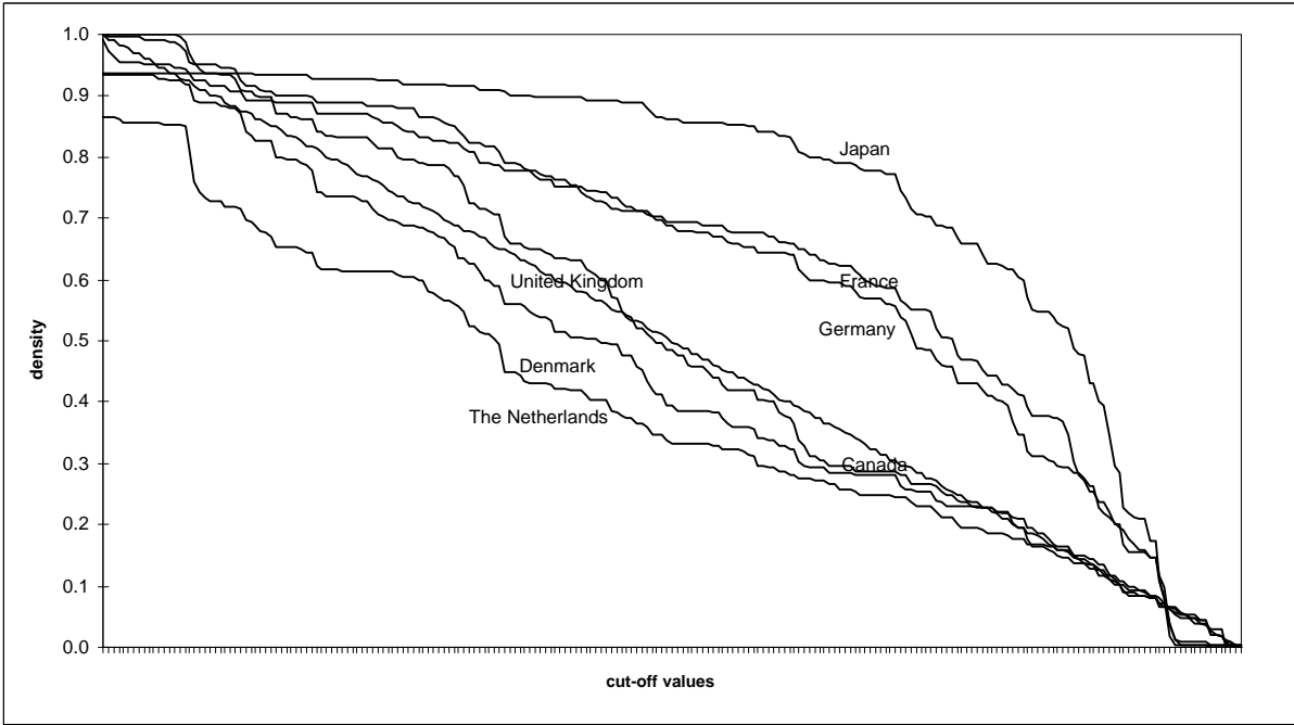
Figure 3.1: Density of the matrices of innovation flows — 1980
