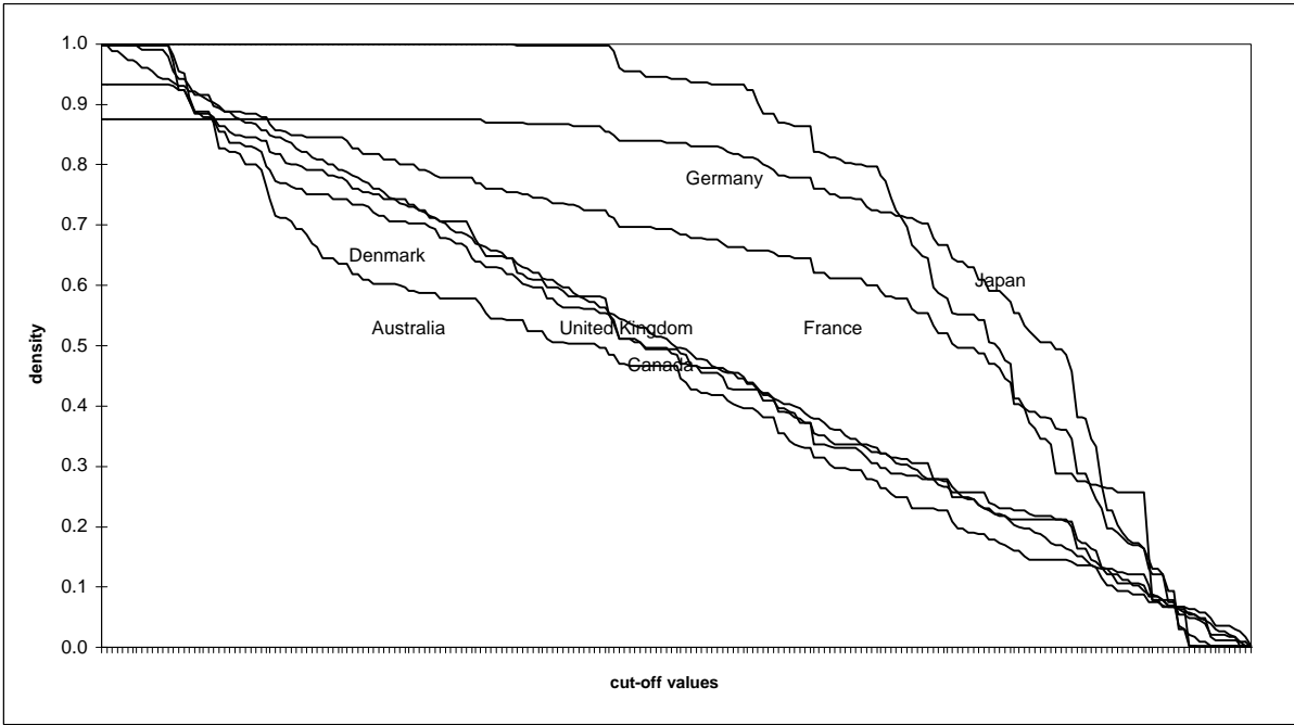
Figure 3.3: Density of the matrices of innovation flows — 1990
