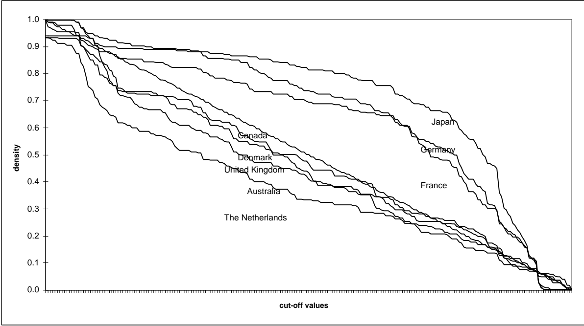
Figure 3.2: Density of the matrices of innovation flows — 1985
