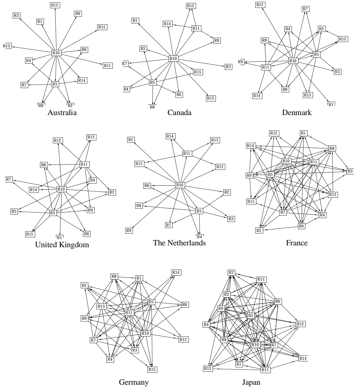
Figure 3.5: Oriented graphs, centrality, 1985
