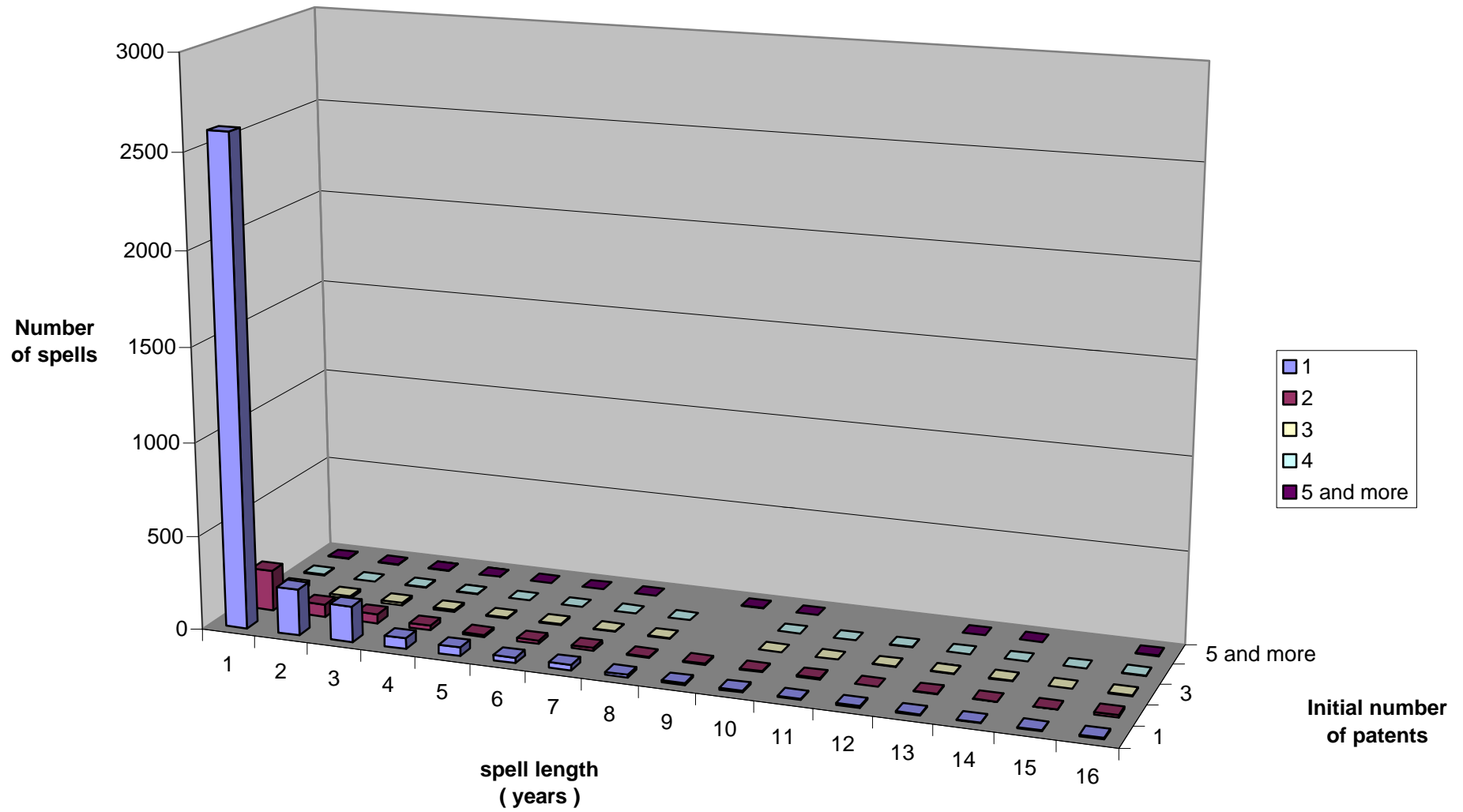
Fig. 4: number of spells, spell length and initial number of patents
