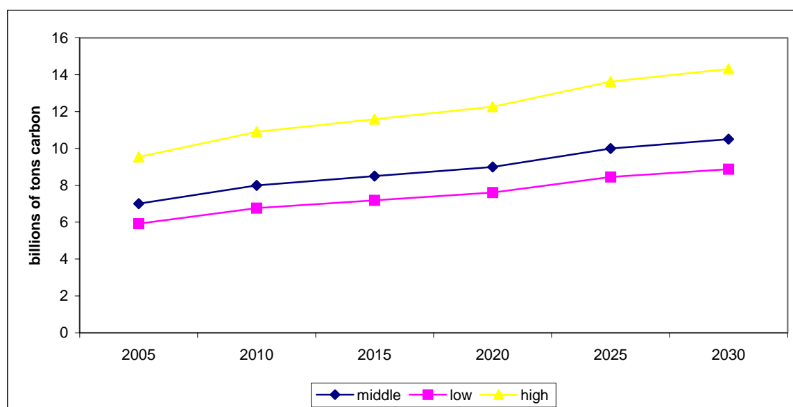
Figure 3: World Carbon emissions paths
